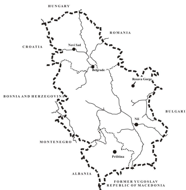
Fig. 1. Geographical position of the Resava Gorge.
