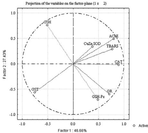
Fig. 4. Principal component analysis (PCA) based on correlations. Projection of all investigated parameters: oxidative stress biomarkers (CuZn SOD, CAT, GSH-Px, GR, GSH, TBARS), bio-transformation phase II enzyme (GST) and acetylcholinesterase activity (AChE) on the factor plane.
