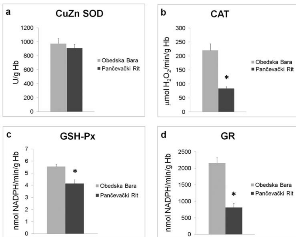
Fig. 2. Comparison of specific antioxidant enzyme activities in snakes from different localities. A – copper-zinc containing superoxide dismutase (CuZnSOD); b – catalase (CAT); c – glutathione peroxidase (GSH-Px); d – glutathione reductase (GR) in RBCs of the dice snake ( Natrix tessellata ) from Obedska Bara and Pančevački Rit. Specific enzyme activities are expressed as U g -1 hemoglobin (Hb). The samples were compared using the Mann-Whitney U -test; (*) significant difference was at p < 0.05 . The number of different specimens used to calculate the means: N=10 for Obedska Bara and N=7 for Pančevački Rit.
