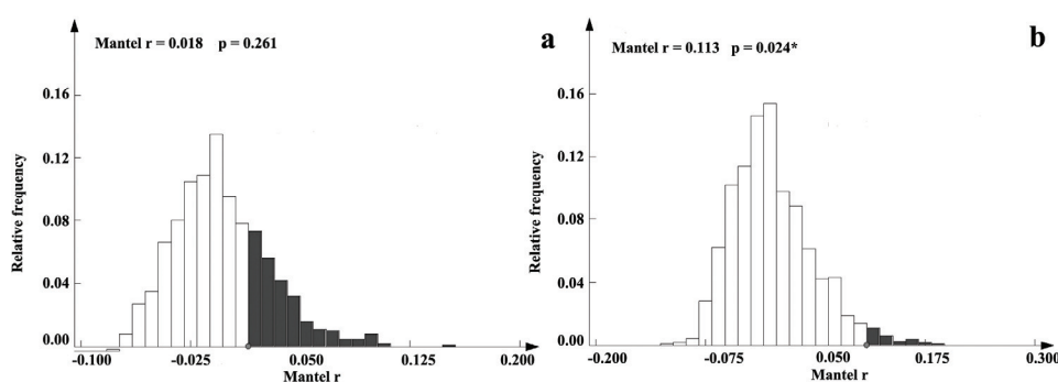
Fig. 1. Overall correlation between the chemistry of soil and birch bark (a) and soil and birch leaves (b).
