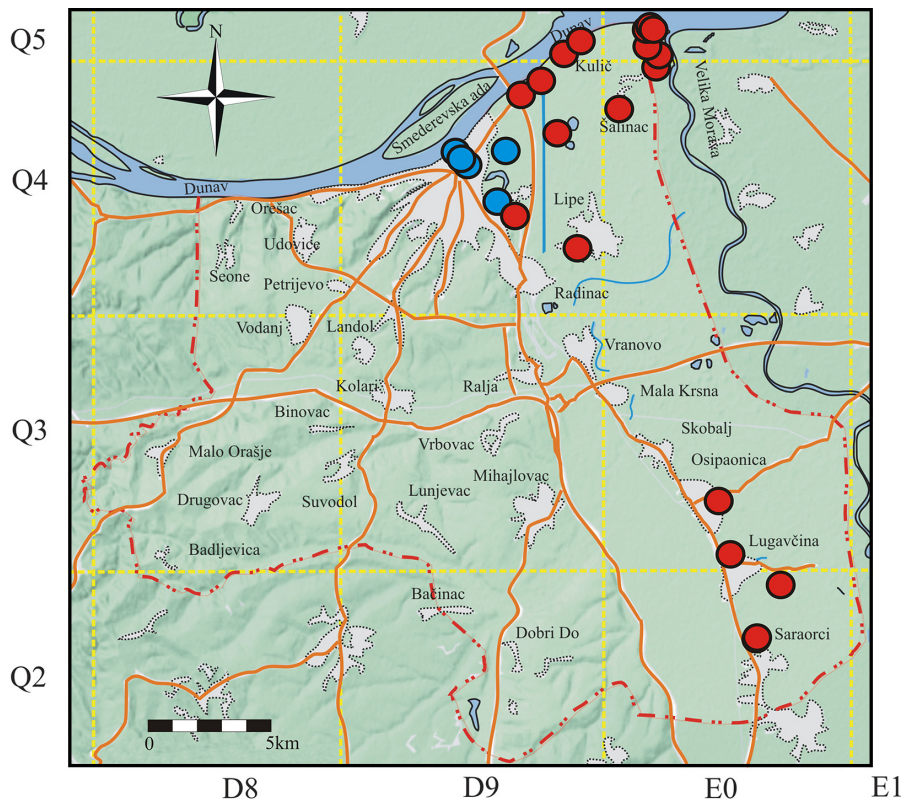
Fig. 14 – Distribution of Emys orbicularis (Linnaeus, 1758) in Smederevo municipality.
