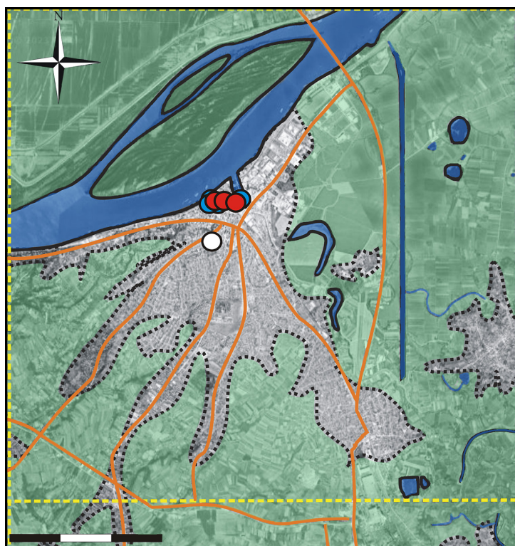
1 3 km Fig. 16 – Distribution of Mediodactylus kotschy (Steindachner, 1870) (blue and red dots) and Pogona vitticeps Ahl, 1927 (white dot) in Smederevo municipality.
