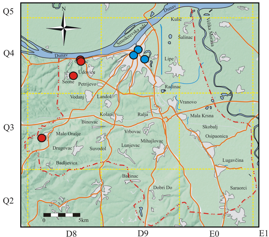
Fig. 2. – Distribution of Salamandra salamandra (Linnaeus, 1758) in Smederevo municipality.
